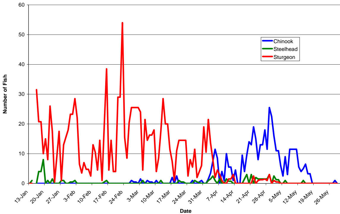
Estimated Chinook, Steelhead, and Sturgeon Take by Steller Sea Lions at Bonneville Dam, 2009
